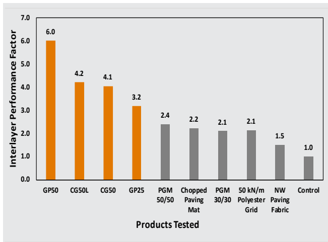
Figure 2: GlasPave Paving Mats interlayer performance factors versus common paving fabrics and mats.
