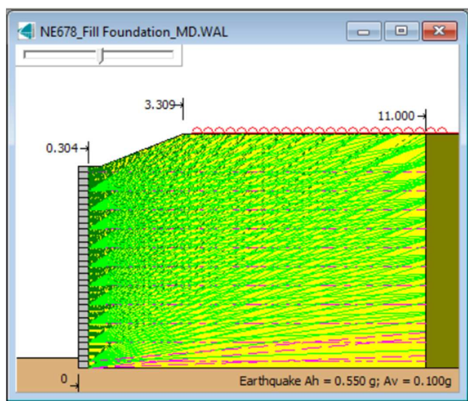
Figure 15. Back-analysis of internal stability
