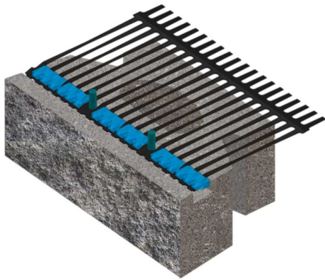
Figure 2. Modular block retaining wall system
