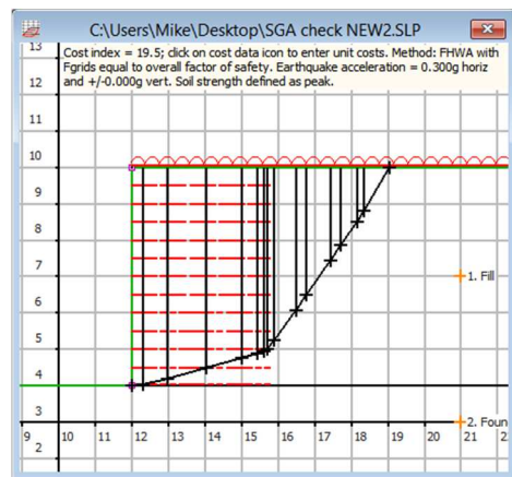
Figure 5. Critical mechanism under seismic loading
