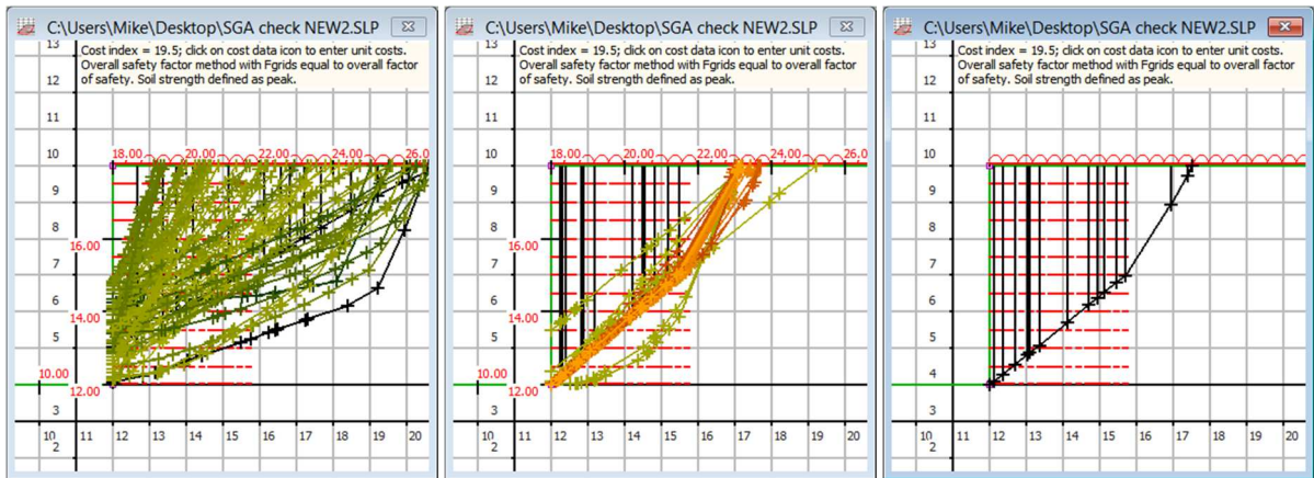
Figure 4. Simplified genetic algorithm process: populate (left), analyse and hunt (middle) and find critical non-circular surface (right).
