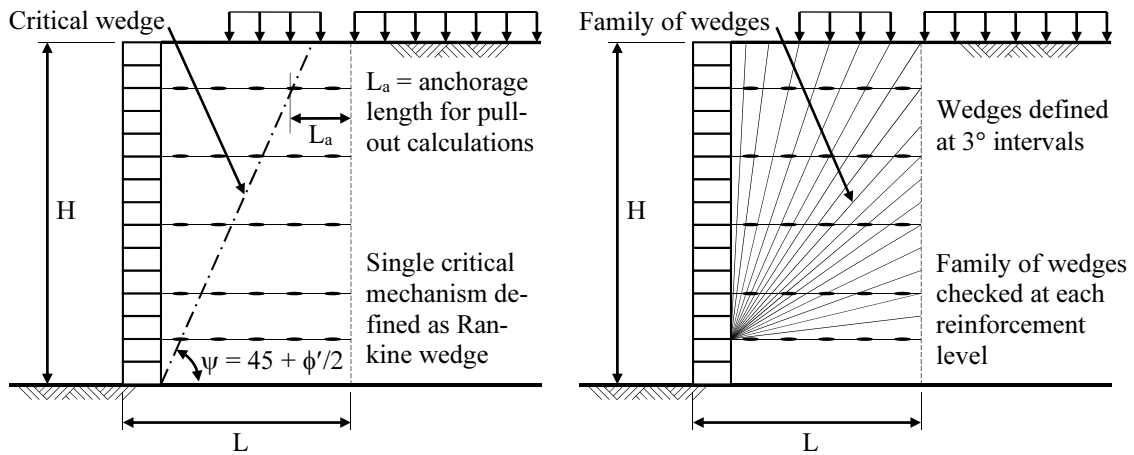
Figure 1. Mechanisms used to check internal stability: tie-back wedge (left) and two-part wedge (right).
