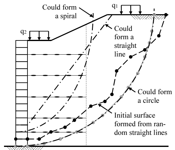
Figure 3. Possible non-circular failure mechanisms
