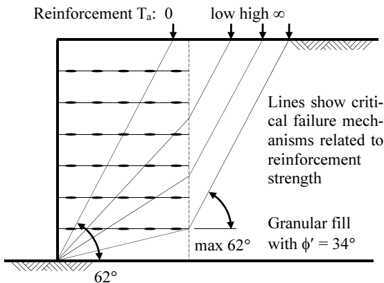
Figure 2. Default failure mechanisms
